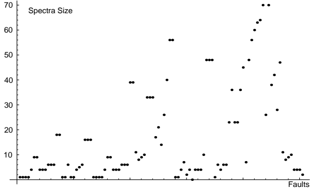
Fig. 2. Spectrum Size Distribution of Stuck-at Faults in 4x4 Multiplier. X Axis: Faults in topological node order. Y Axis: Spectrum size
